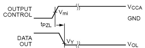
Figure 6. 3-STATE Output Low Enable Time (18)
