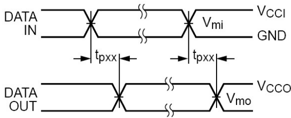
Figure 5. Waveform Inverting and Non-Inverting Functions (18)
