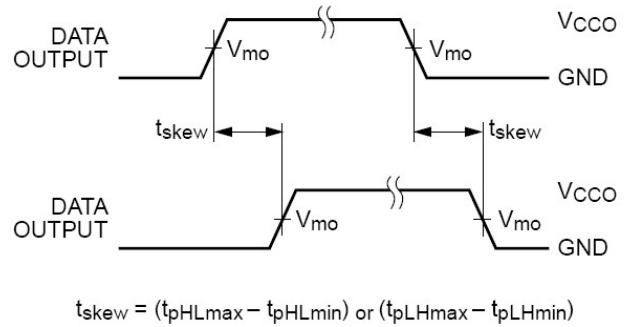
Figure 11. Output Skew Time
