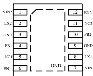
DFN3X3-12 (HM5202)
